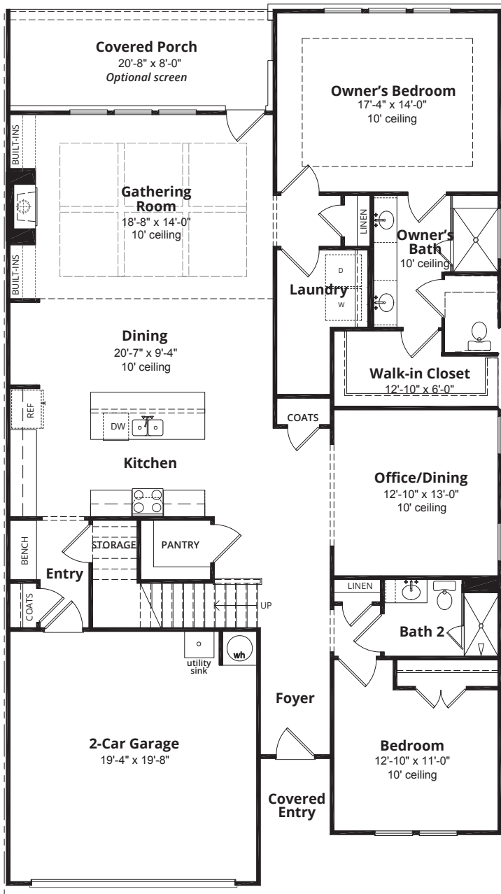
FIRST FLOOR 2,017 finished sq. ft.
